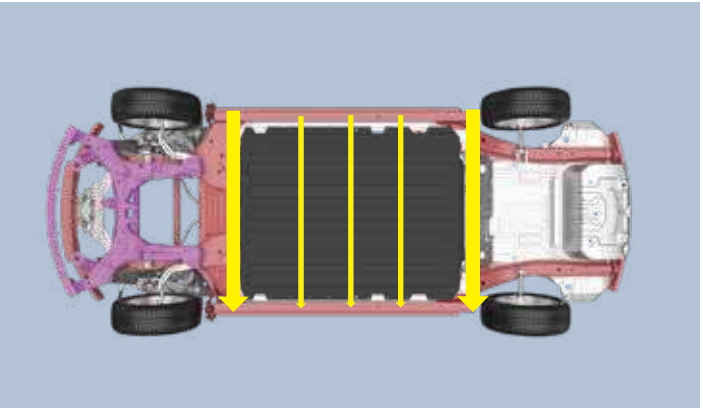
Side-impact 30% battery force transmission*
